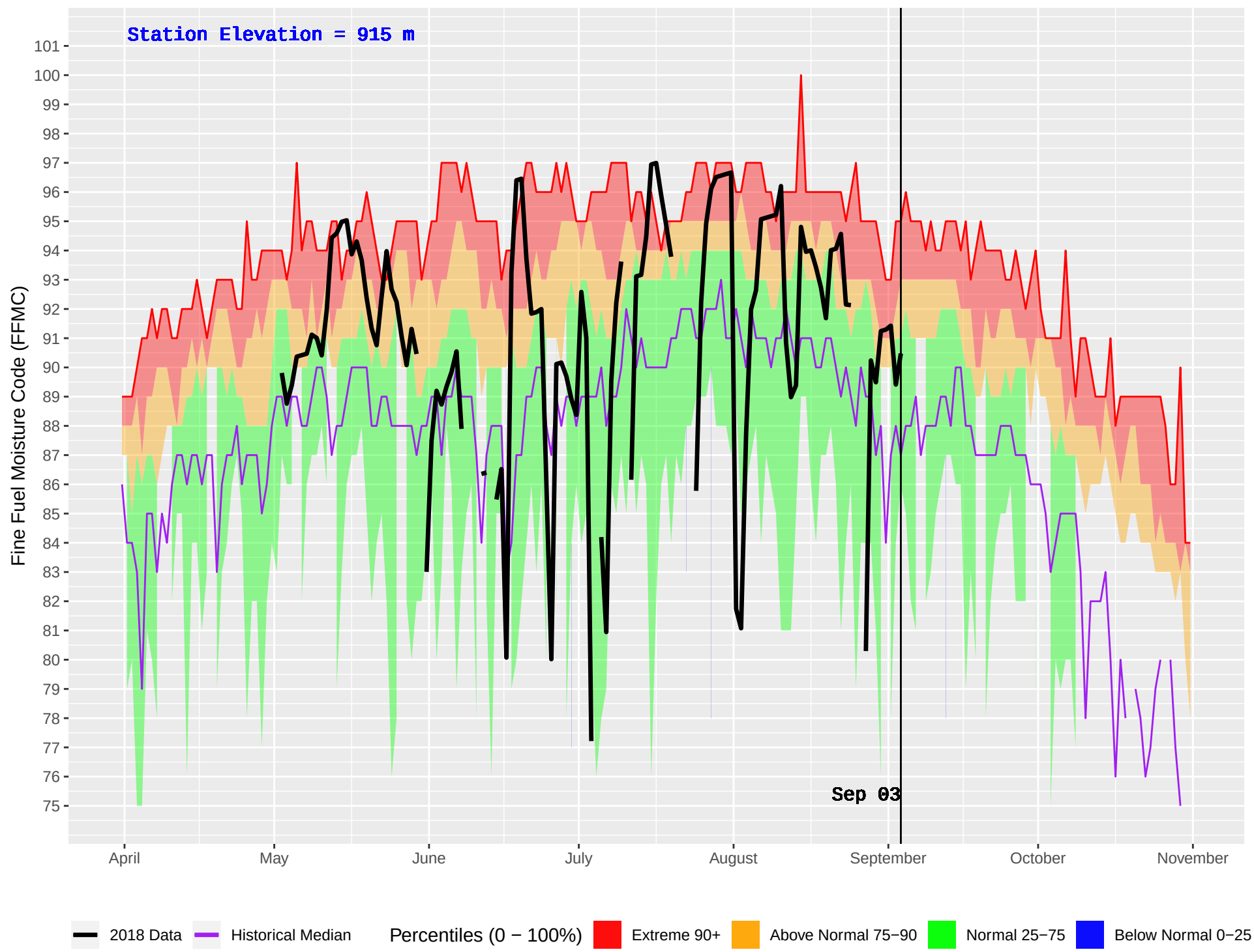
MIDDLE LAKE (226) : Historical (1989–2016) and Current (2018) Daily Fine Fuel Moisture Code (FFMC)
