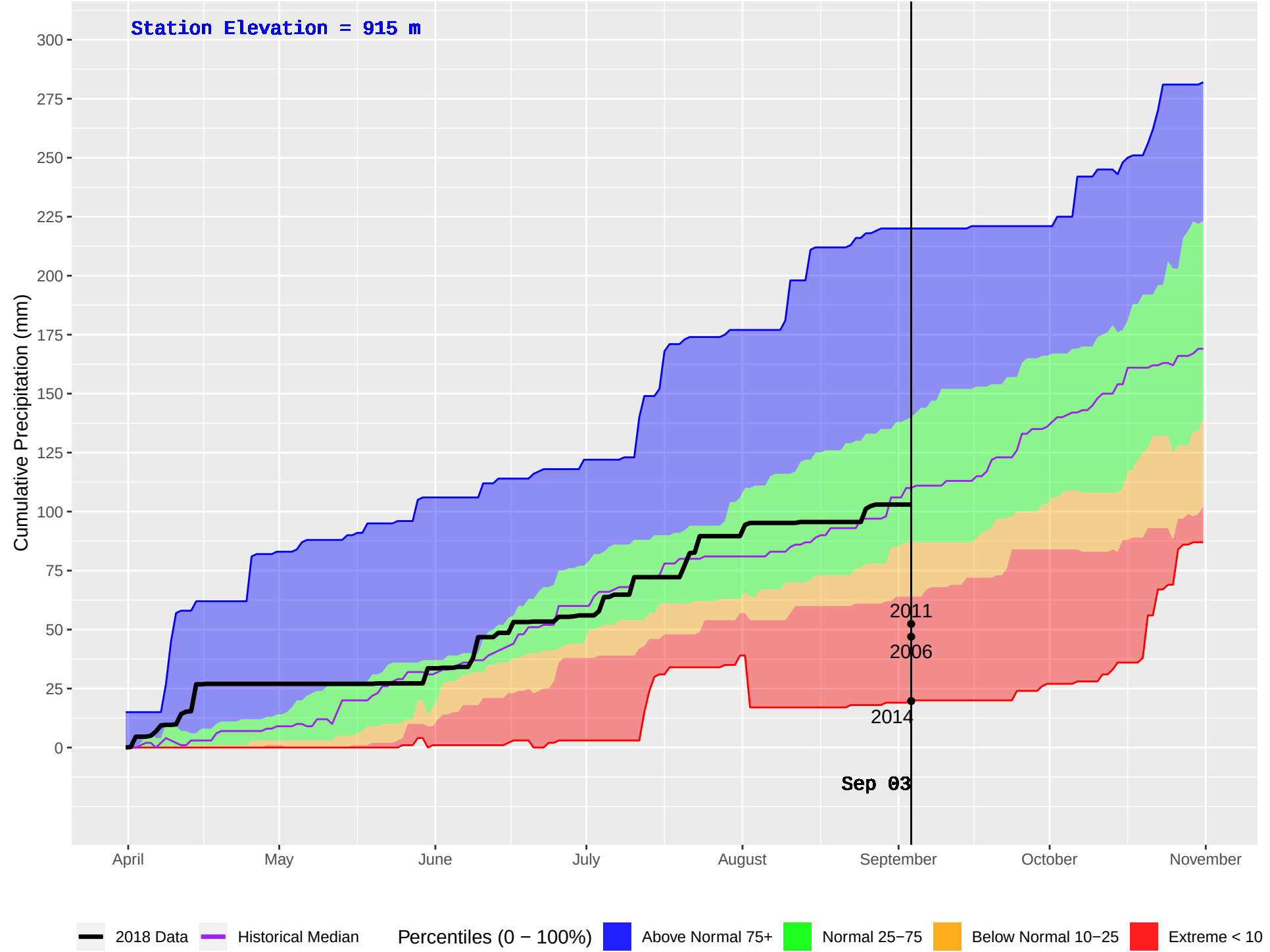
MIDDLE LAKE (226) : Historical (1989–2016) and Current (2018) Daily Cumulative Precipitation
