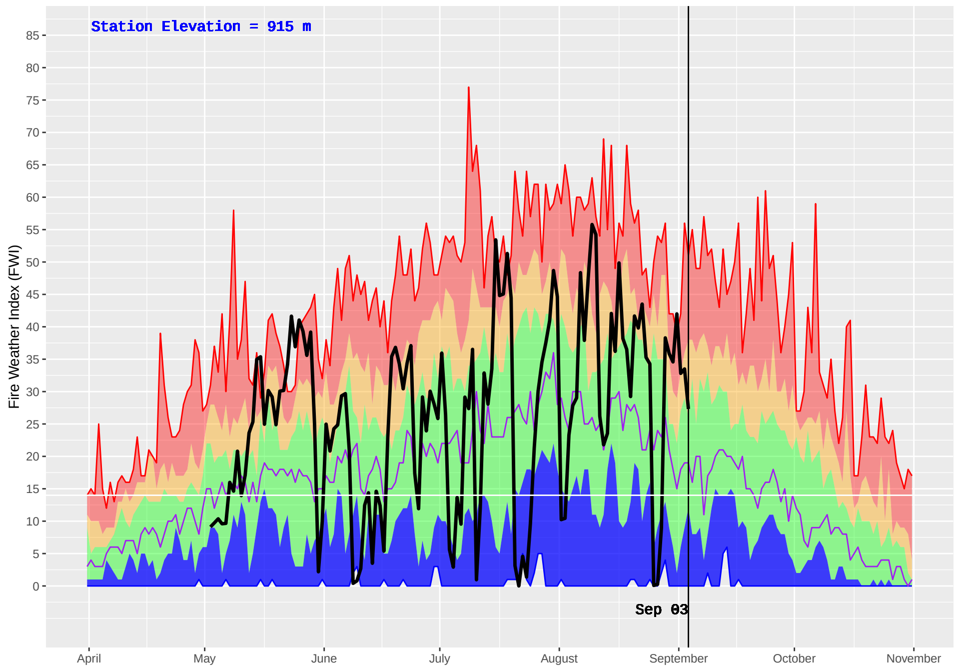
MIDDLE LAKE (226) : Historical (1989–2016) and Current (2018) Daily Fire Weather Index (FWI)
