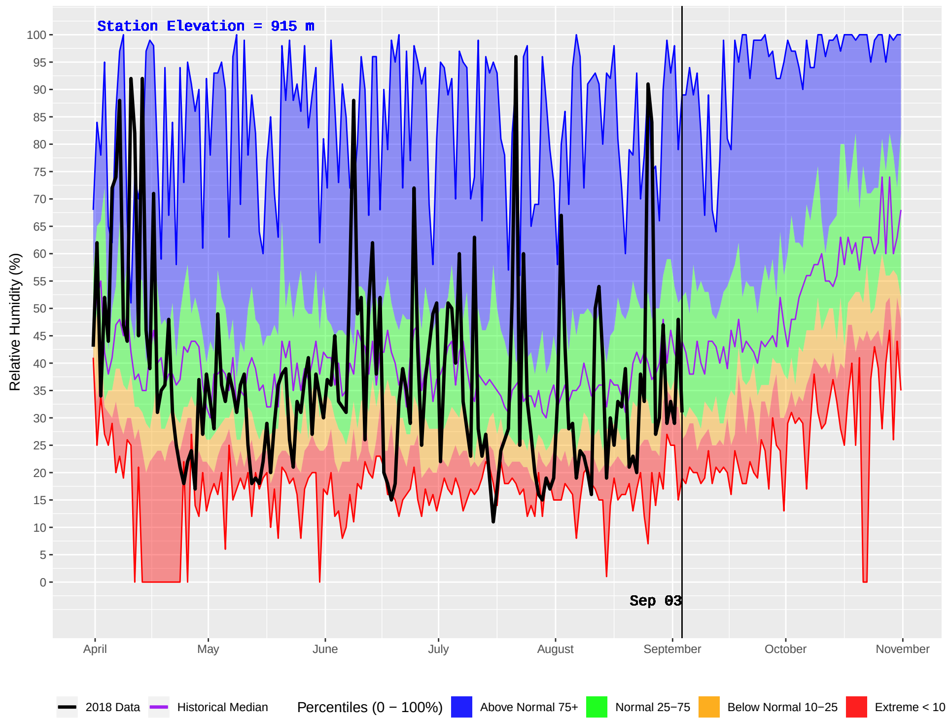
MIDDLE LAKE (226) : Historical (1989–2016) and Current (2018) Daily Relative Humidity
