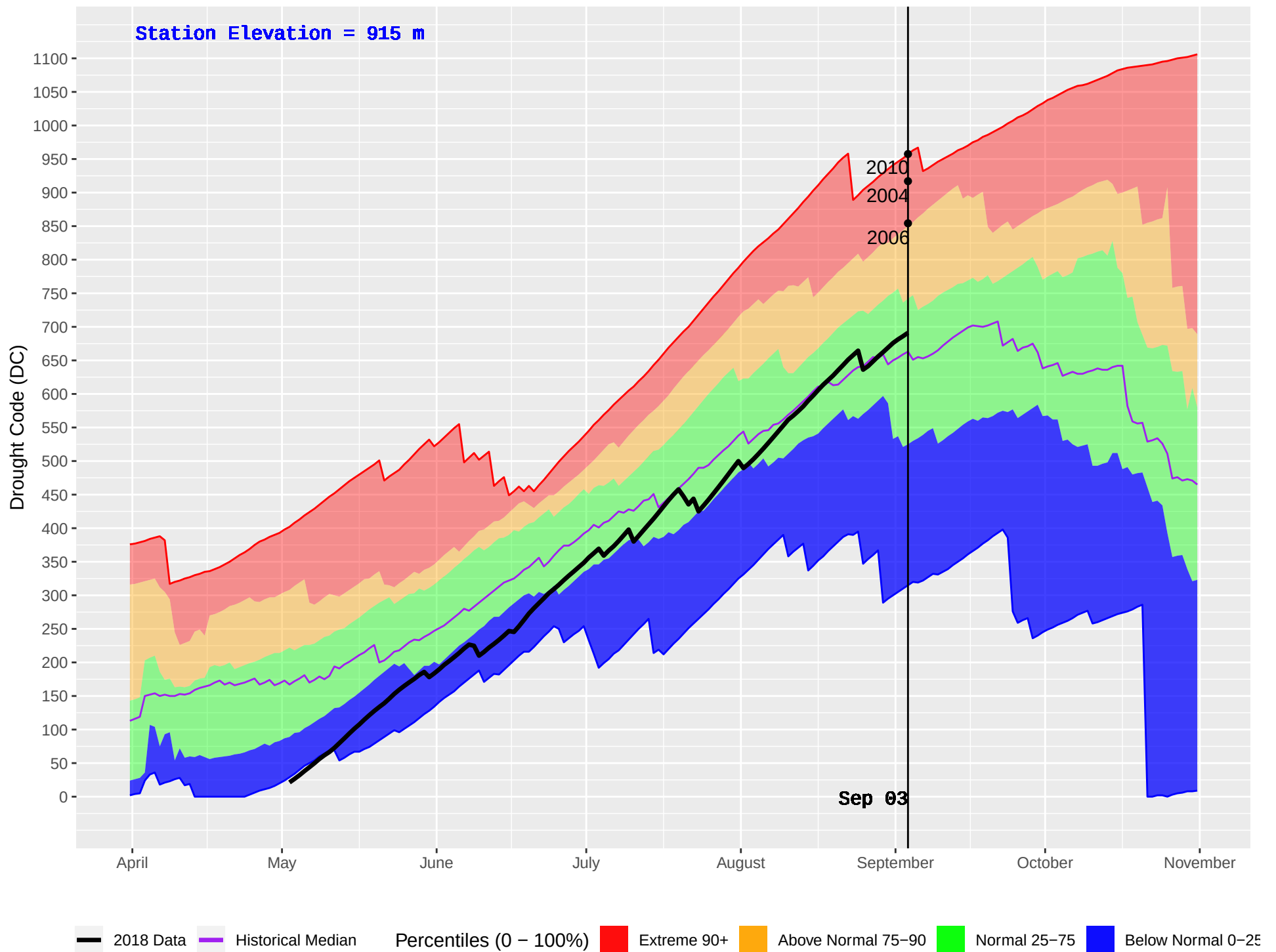
MIDDLE LAKE (226) : Historical (1989–2016) and Current (2018) Daily Drought Code (DC)
