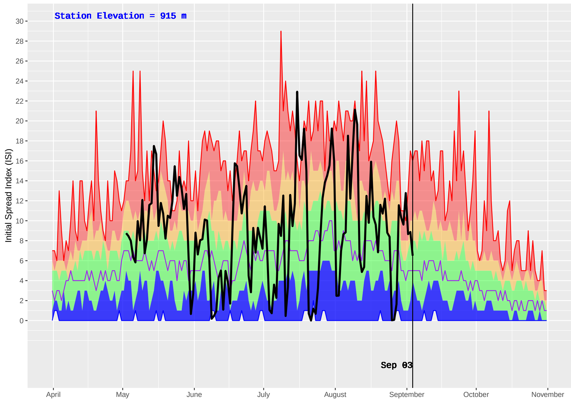
MIDDLE LAKE (226) : Historical (1989–2016) and Current (2018) Daily Initial Spread Index (ISI)
