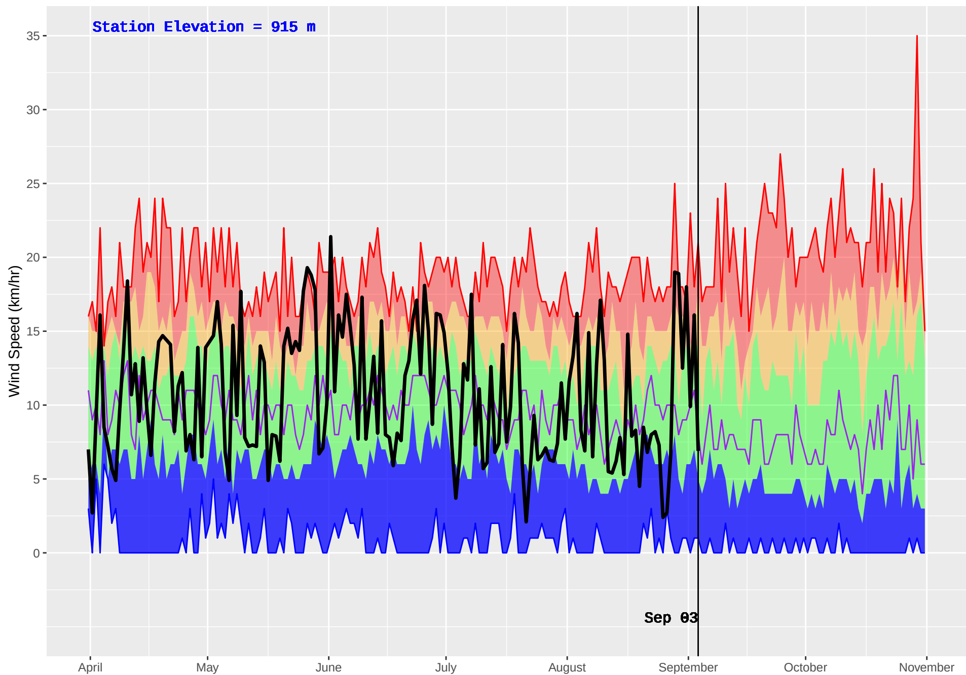
MIDDLE LAKE (226) : Historical (1989–2016) and Current (2018) Daily Wind Speed
