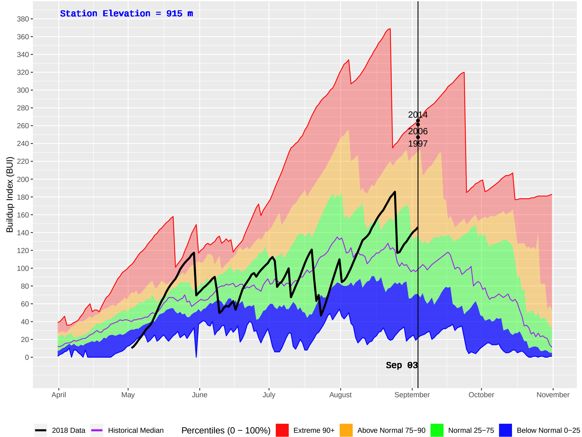
MIDDLE LAKE (226) : Historical (1989–2016) and Current (2018) Daily Buildup Index (BUI)
