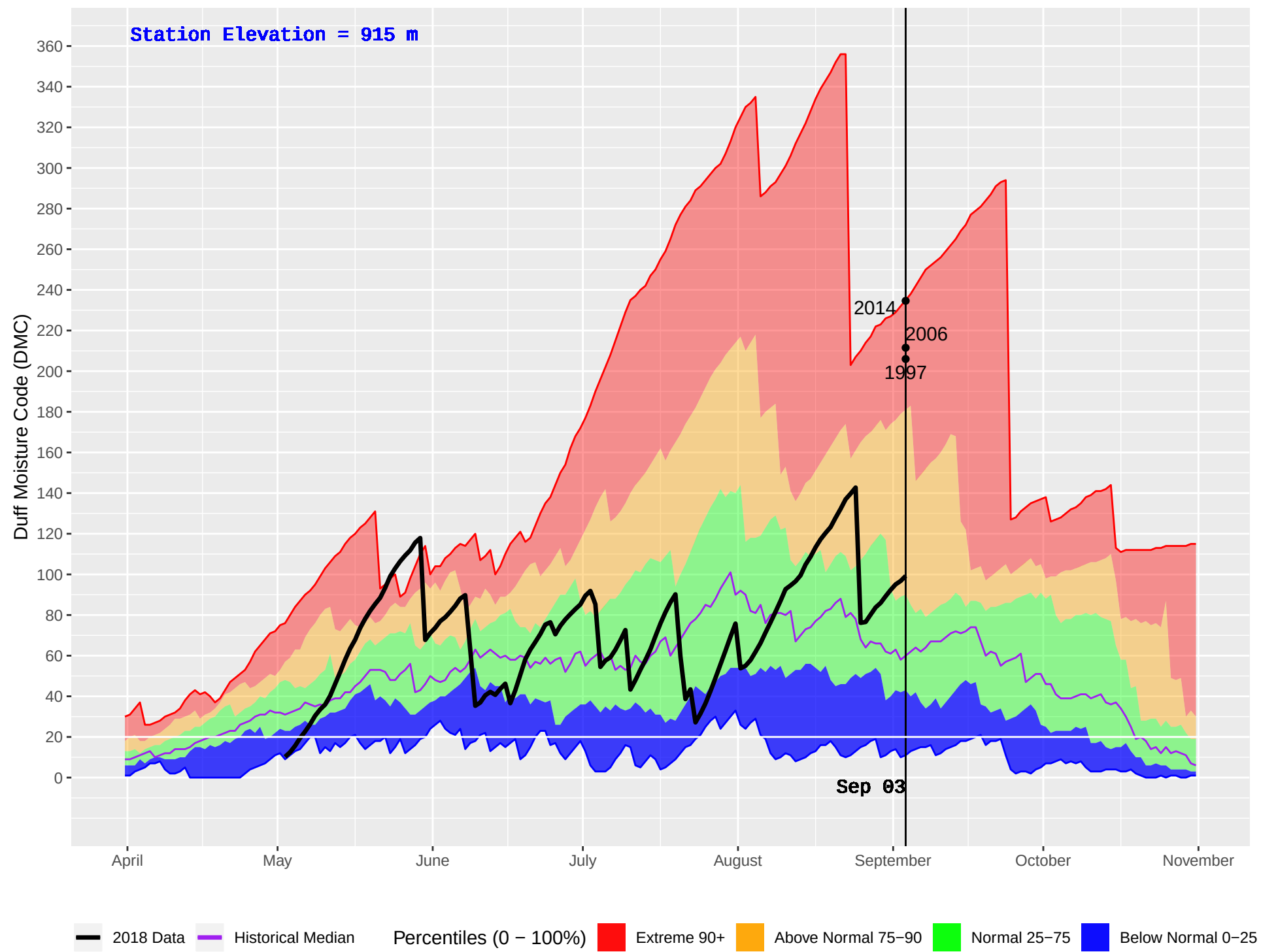
MIDDLE LAKE (226) : Historical (1989–2016) and Current (2018) Daily Duff Moisture Code (DMC)
